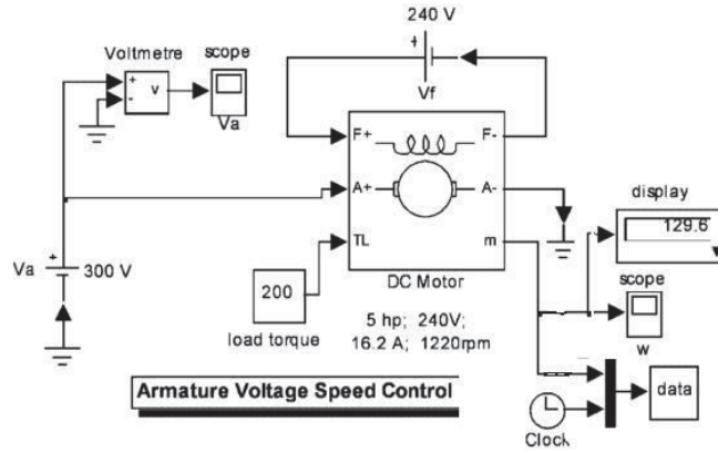
Figure 2 Simulink implementation of armature voltage speed control method.
