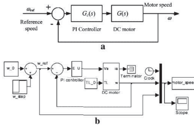
Figure 3 Feedback control system for DC motor speed control: (a) block diagram; (b) Simulink model.
