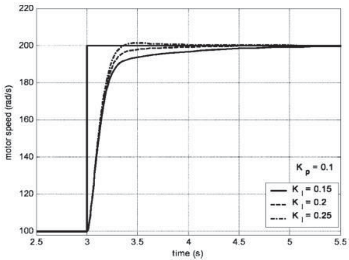
Figure 9 Motor speed for different PI gain values.
